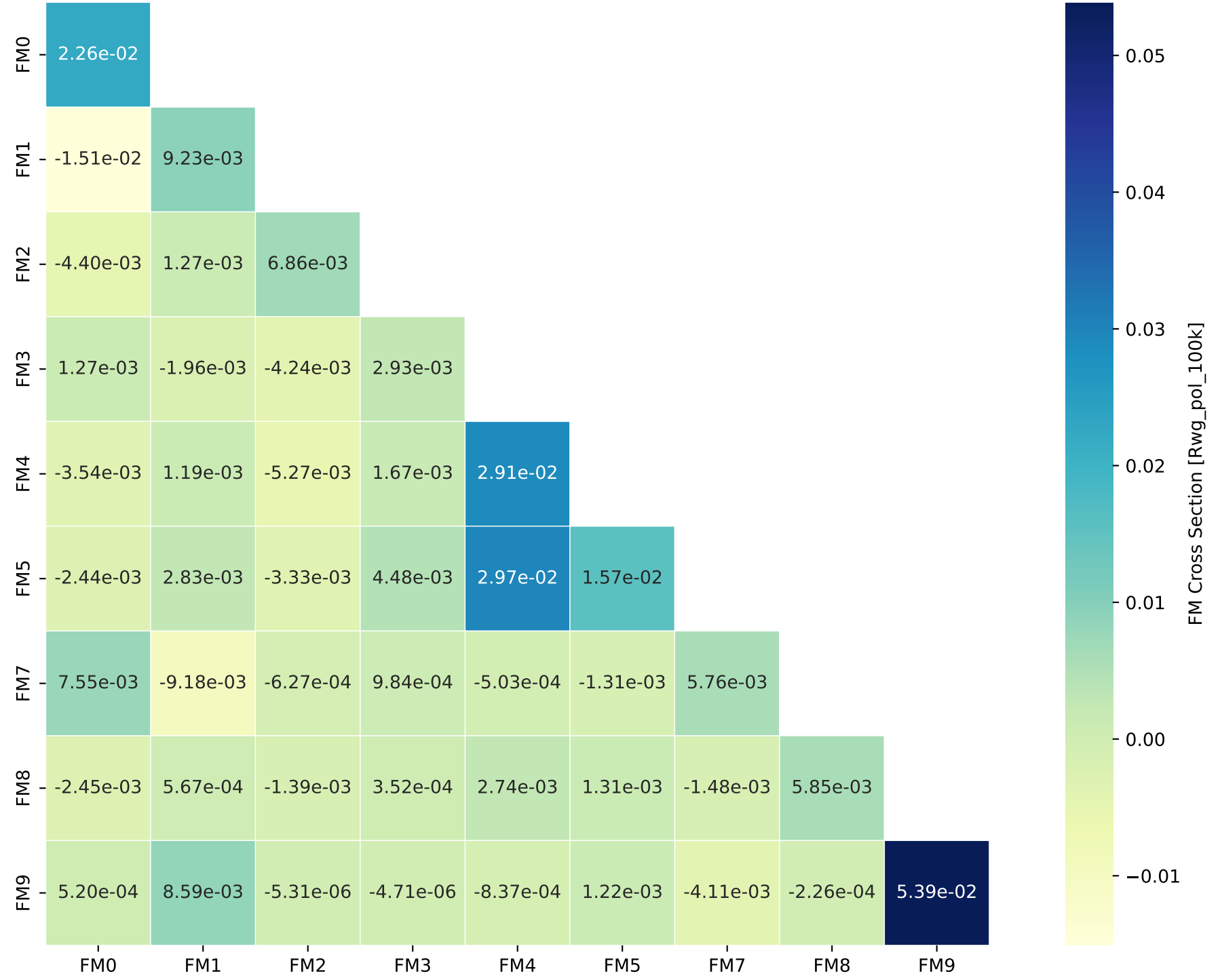
FM Cross Section [Rwg_pol_100k]
